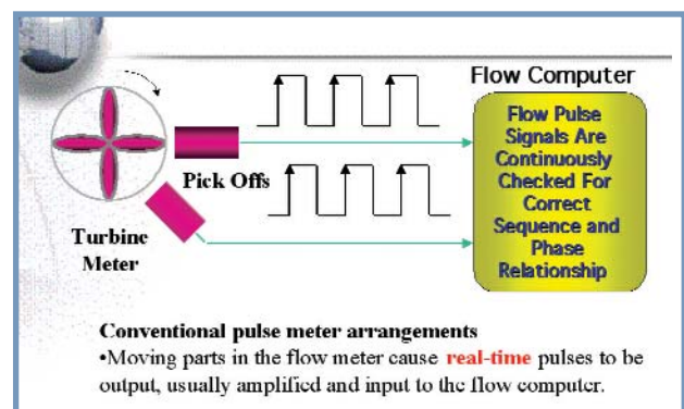
Conventional real-time meter pulses.
