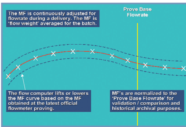
Meter factor linearisation using flowrate and viscosity.
