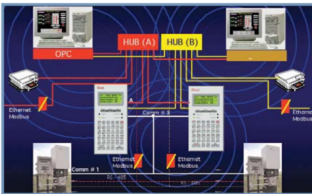
LAN network and communication ports.
