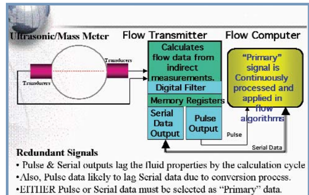
Fidelity or redundant signals?
