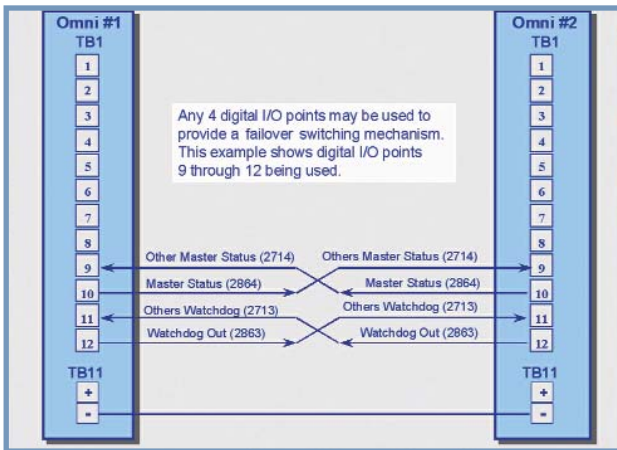
Implementing redundant flow computers.
