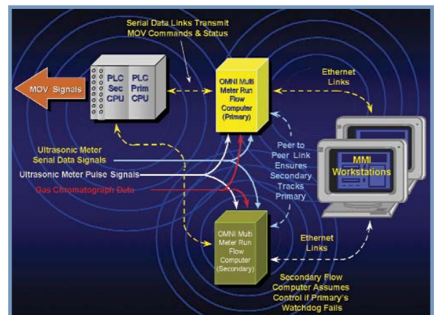
Redundant electronic system components.
