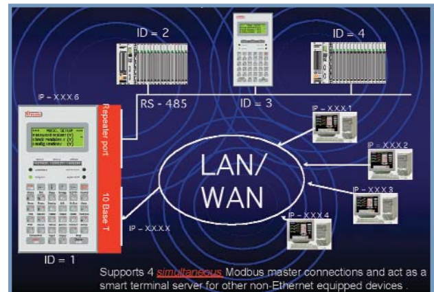
Ethernet equipped flow computers.
