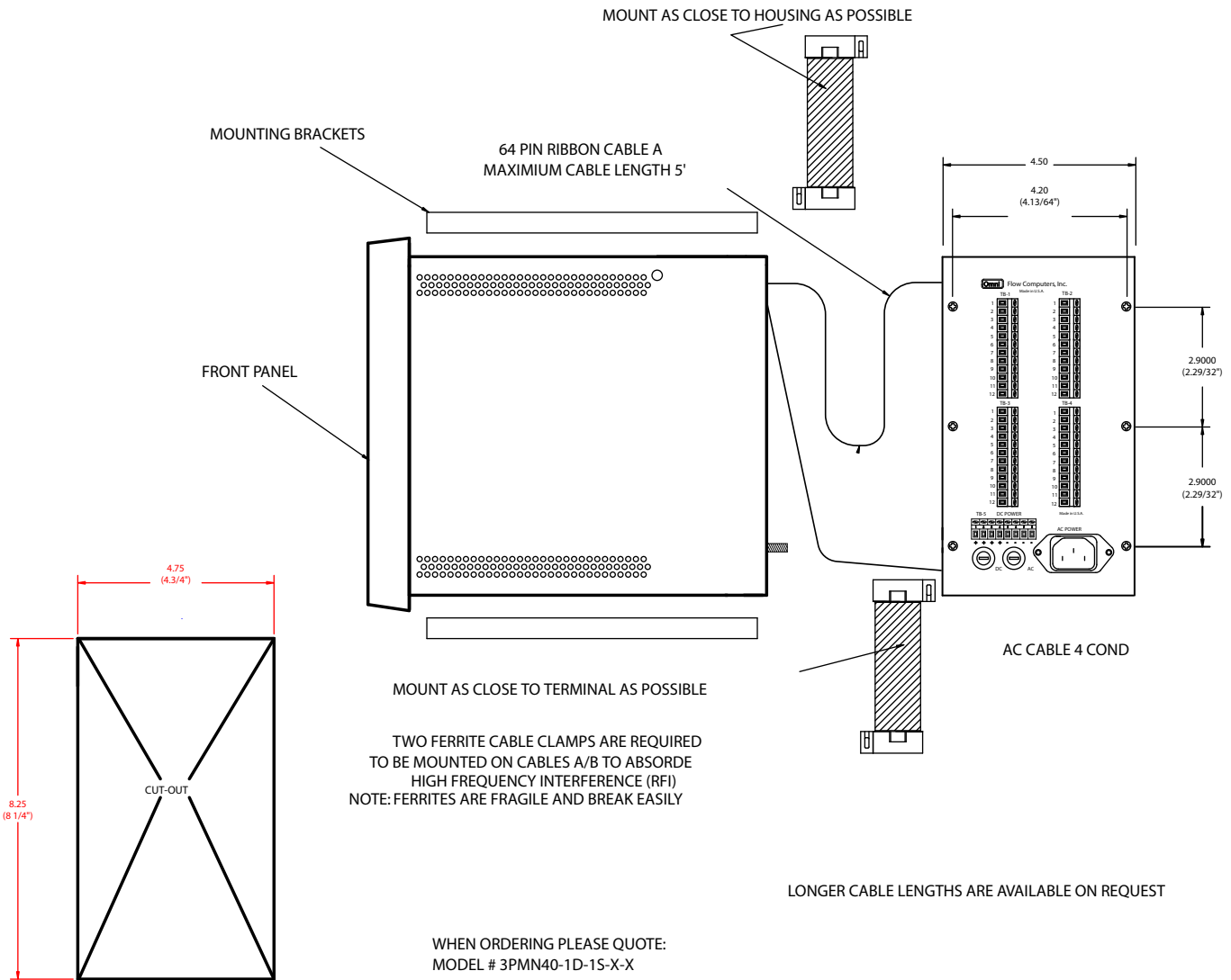
PANEL CUT OUT DIMENSIONS
