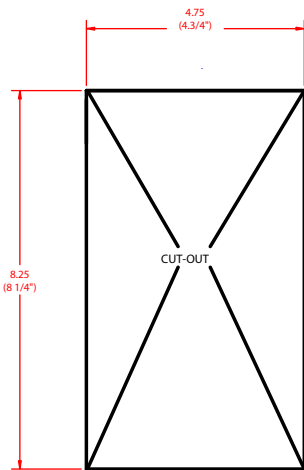
PANEL CUT OUT DIMENSIONS
